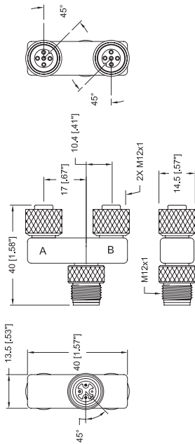
ASBS 2 M12-S2326
